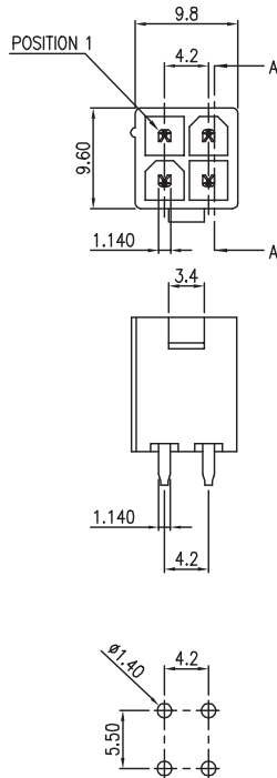
RECOMMENDED PCB LAYOUT
