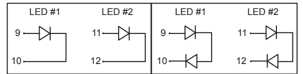
Single Color LED Bi-Color LED
