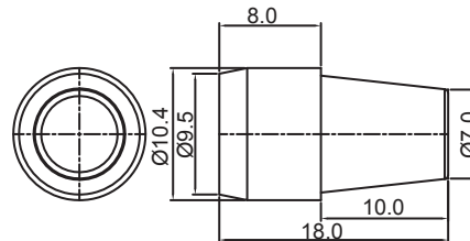
STRAIN RELIEF
