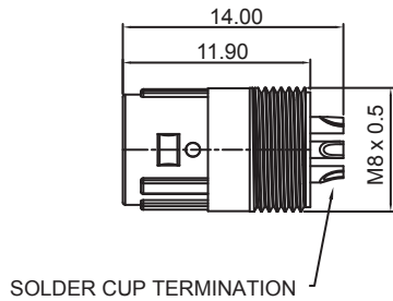
HOUSING+CONTACT+SHELL A
