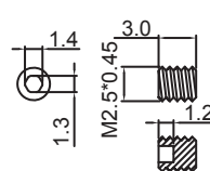
SCREW
