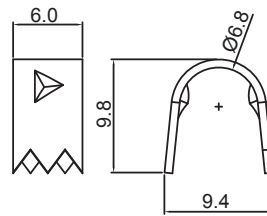
CLAMP
