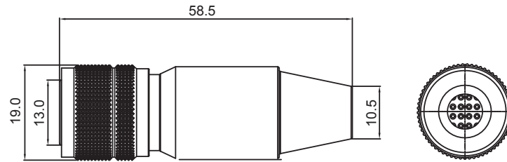
SHELL B + SHELL C + SPRING
