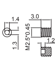
SCREW
