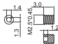
SCREW
