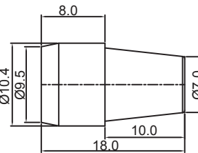
STRAIN RELIEF
