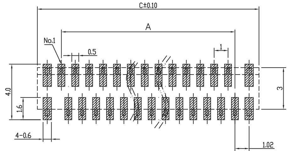
RECOMMENDED PCB LAYOUT (COMPONENT SIDE)
