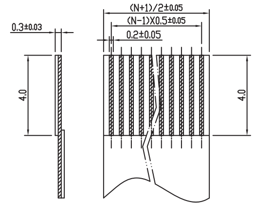
FFC/FPC DIMENSION
