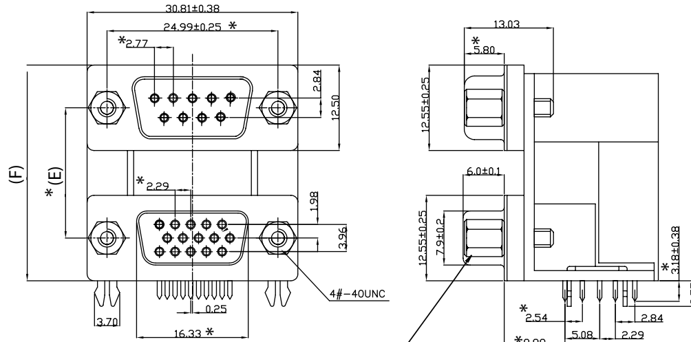
Hardware - Shown with Jackscrews Installed
